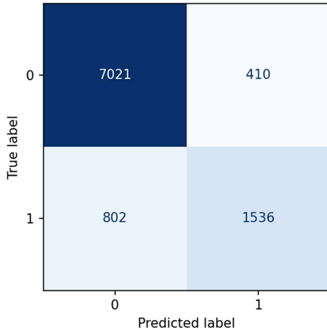
Adult Income – XGBoost Confusion Matrix
